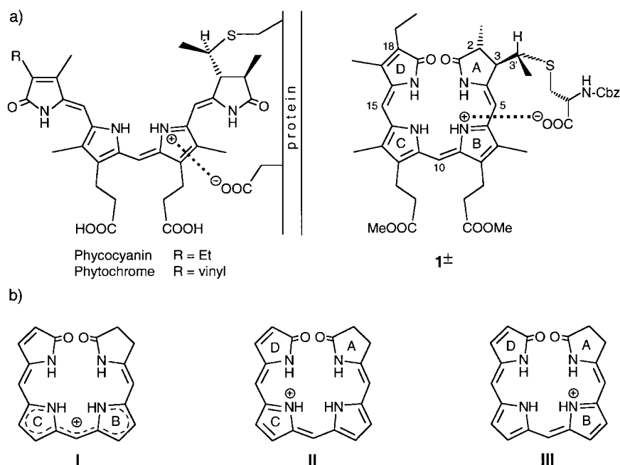
Figure 1. a) Comparison of the extended ( Santi,10syn,14anti ) conformation of the protein-bound chromophores of phycocyanin and the Pr form and the helical ( 5syn,10syn,14syn )-conformation of model compound 1 in its zwitterionic form 1 ± . b) Hypothetical chromophore structures of protonated 2,3-dihydrobilindiones.
